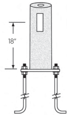
SBR elevation See recommended "capping detail"
