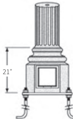
21CT Base plate elevation
