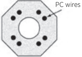
9CT shaft cross-section detail
