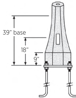
Elevation See recommended "capping detail"
